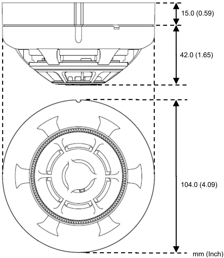
Figure 1: Dimension of EVA-PYH3
