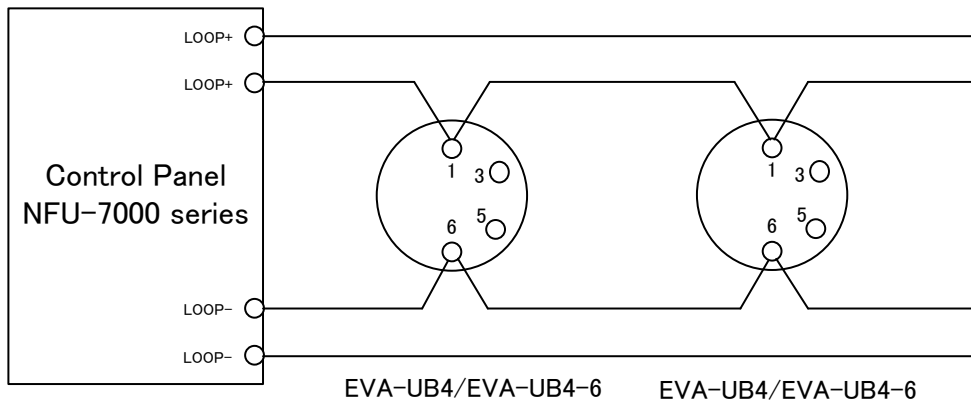
Figure 18: Wiring diagram for EVA-UB4 and EVA-UB4-6
