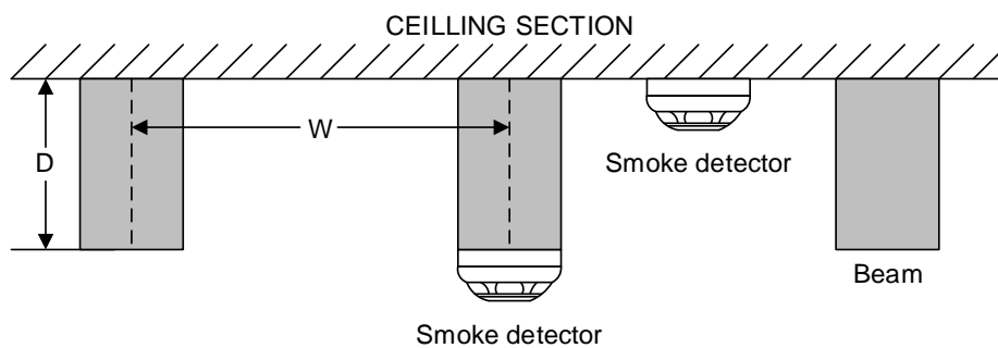
Figure 16: Smoke detector spacing — beam construction (side view)
